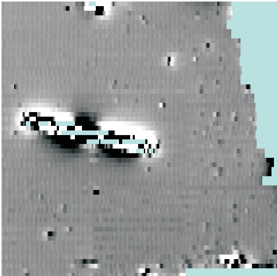
Magnetic gradiometer survey: +/-20nT
