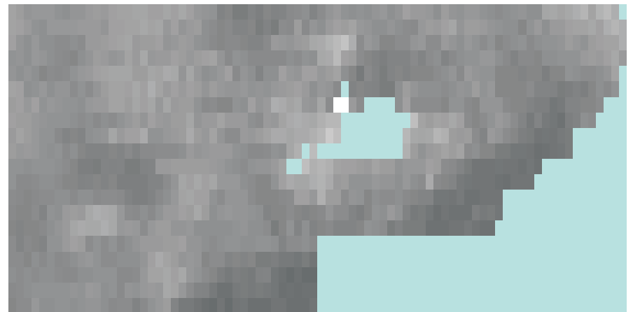
Ground resistivity (shallow - 0.5m spacing) greyscale 62Ω black to 312Ω white measured resistance
